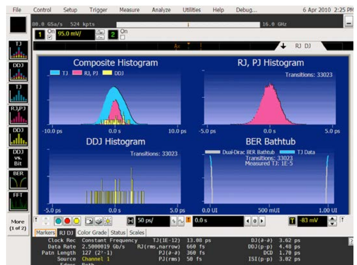
Jitter separation makes debugging your device easy
