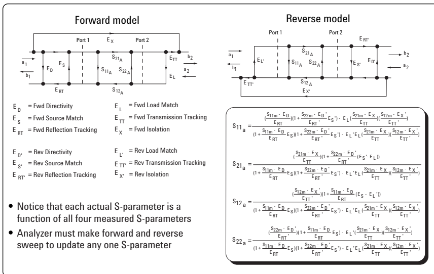
Figure 5. Two-Port Error Correction
