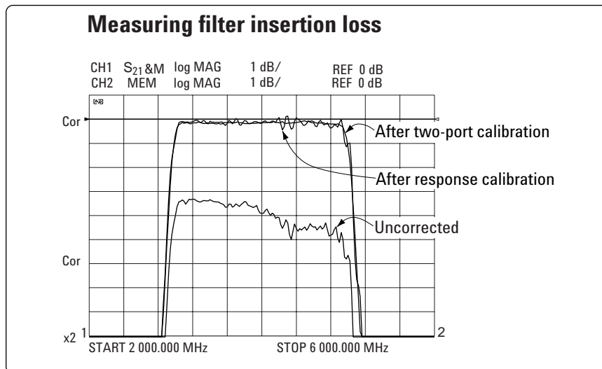
Figure 1. Response versus Two-Port Calibration
