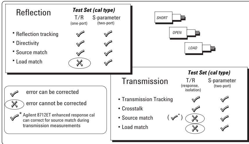
Figure 7. Calibration Summary
