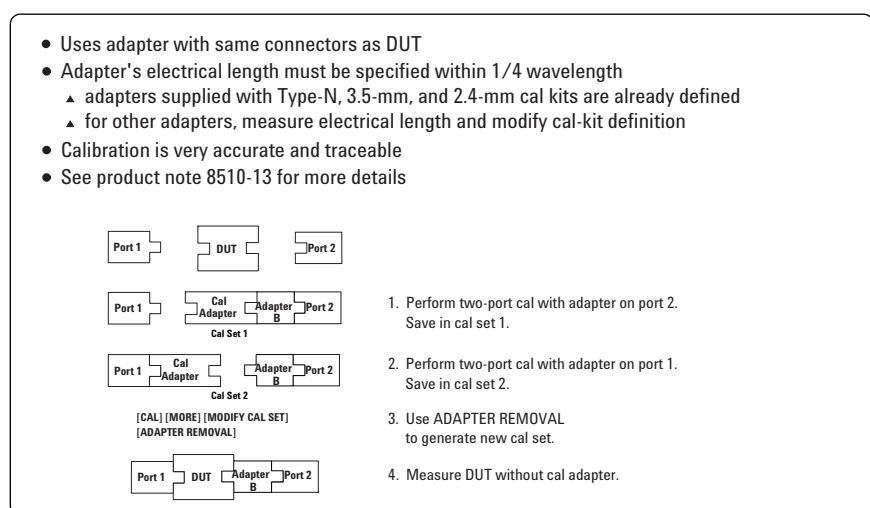
Figure 16. Adapter-Removal Calibration
