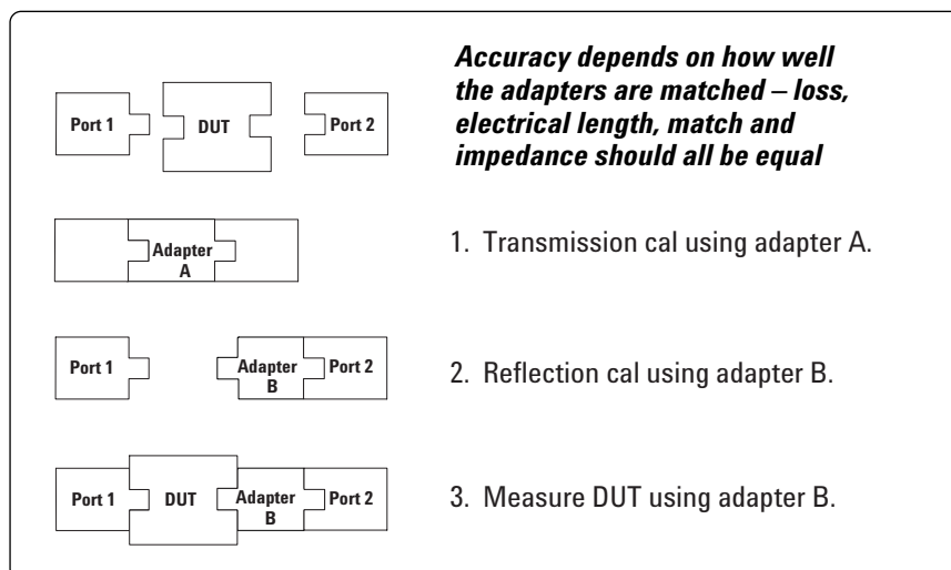
Figure 15. Swap-Equal-Adapters Method
