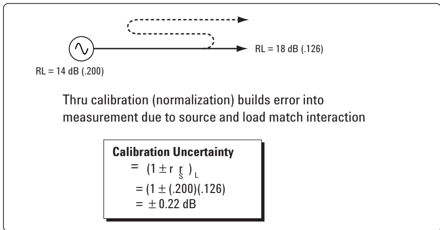
Figure 10. Transmission Example Using a Response Cal
