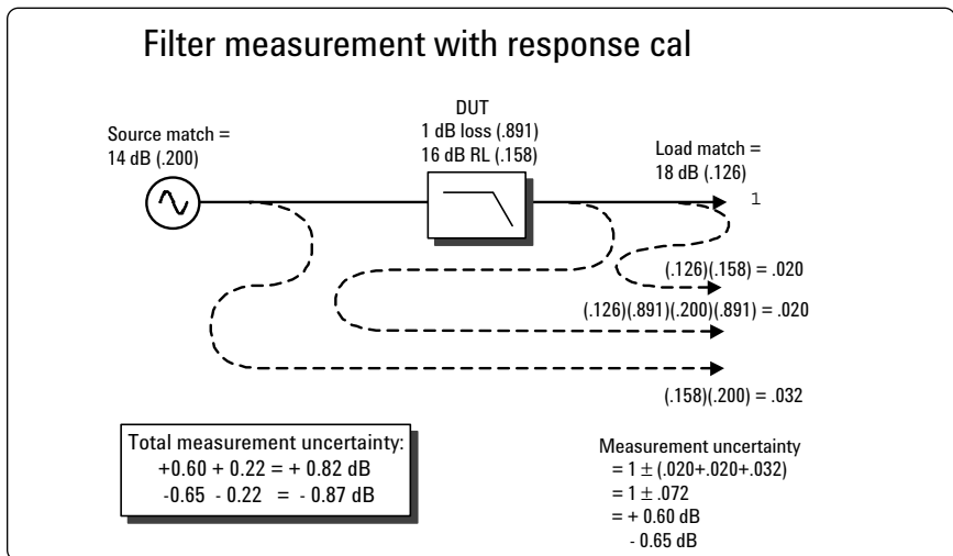
Figure 11. Transmission Example (continued)
