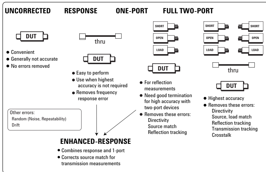
Figure 6. Errors and Calibration Standards
