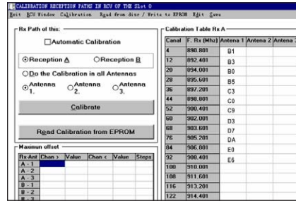
Figure 2. Base Station RX Level Calibration Software
