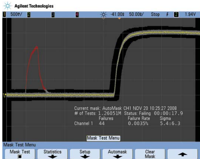
Figure 6: Mask testing to 6.3σ resolution takes only seconds using an InfiniiVision scope with an update rate of 100,000 waveforms per second
