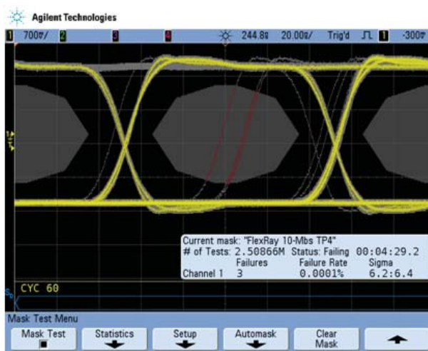
Figure 4: Mask testing lets you specify areas around your signal that should be off limits
