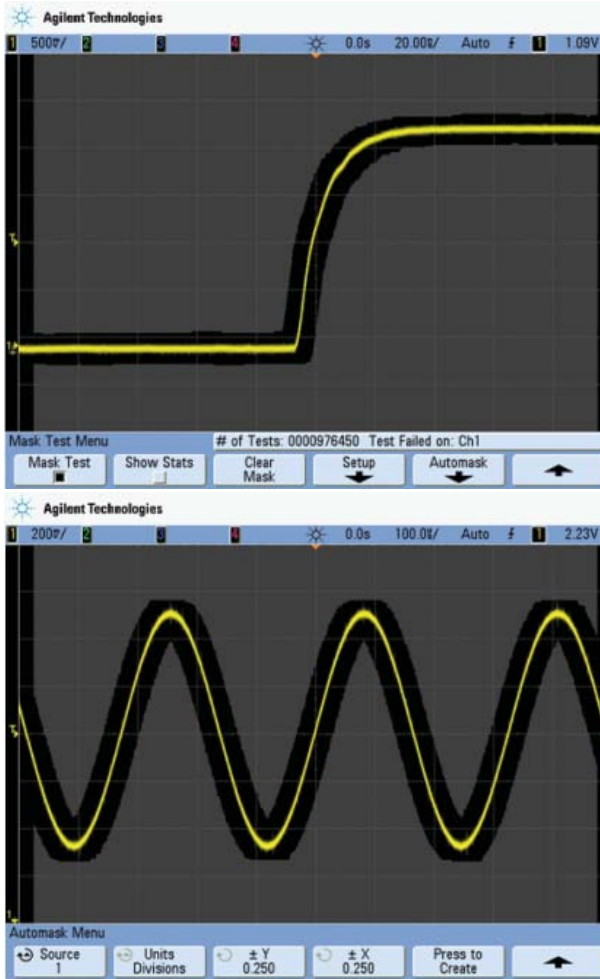
Figure 3: Mask testing compares your signal with correct signal and alerts you if your signal passes outside specific limits
