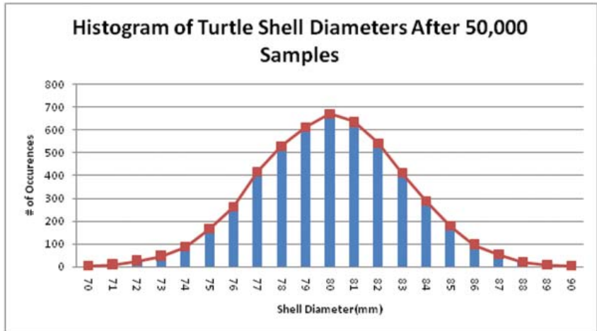
Figure 1: After 50000 samples, the histogram of turtle shell diameters acquires a curved shape
