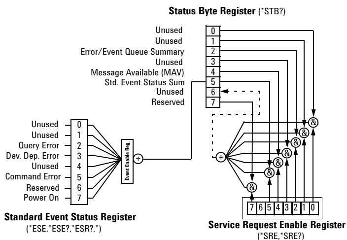
Figure 1 Agilent N9320B Status Register System
