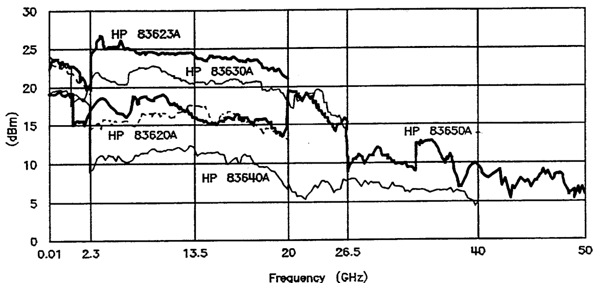
Typical Maximum Available Power
