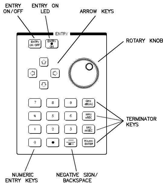
Figure 1-3. Entry Area
