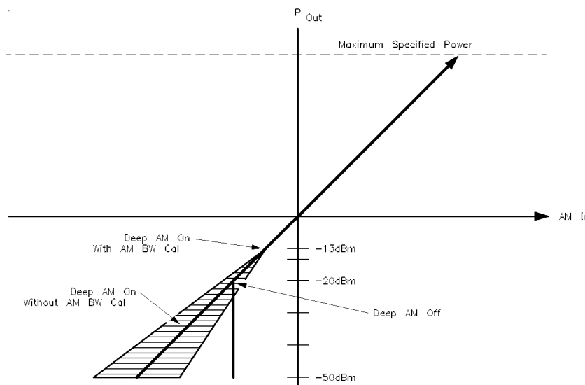
Figure M-2. Power Accuracy Over the AM Dynamic Range
