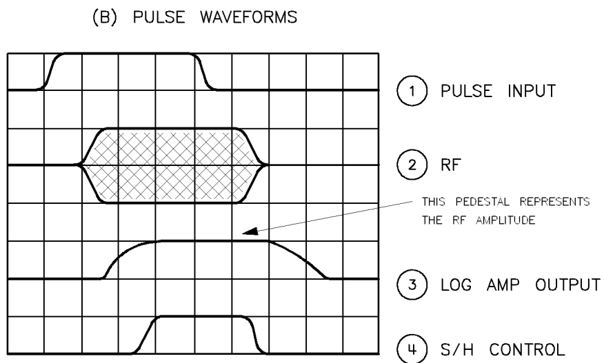
Figure M-5. Pulse Modulation System
