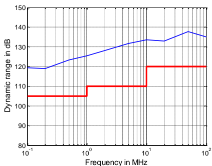
Dynamic range in dB versus frequency for the R&S®ZNB26/40.
