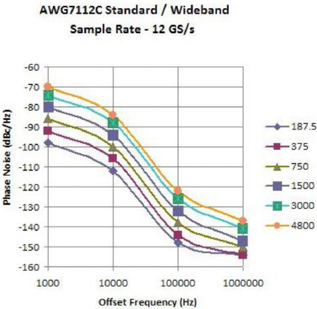
AWG7122C Interleave Phase Noise (typical).
