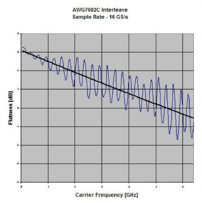
AWG7082C Interleave Flatness (typical).
