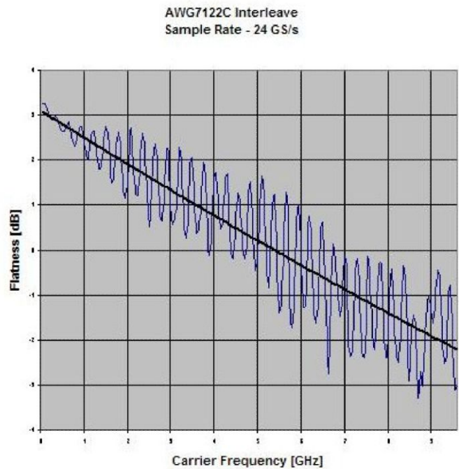
AWG7122C Interleave Flatness (typical)
