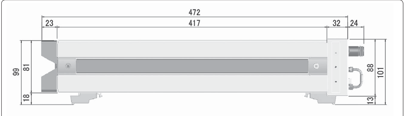
Figure 14. Dimensions (side view, with Option E5091A-016, in millimeters, nominal)
