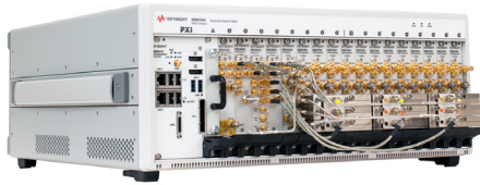
Figure 5. 12-port configuration
